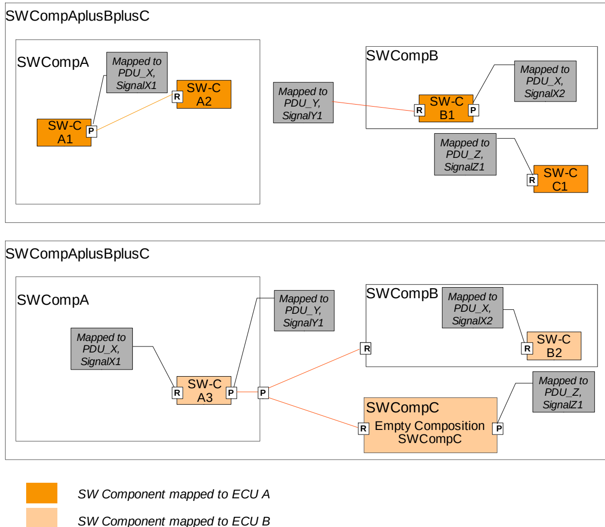
Figure 9.4: Example System extract for ECU A (upper figure) and ECU B (lower figure) of above introduced composition
