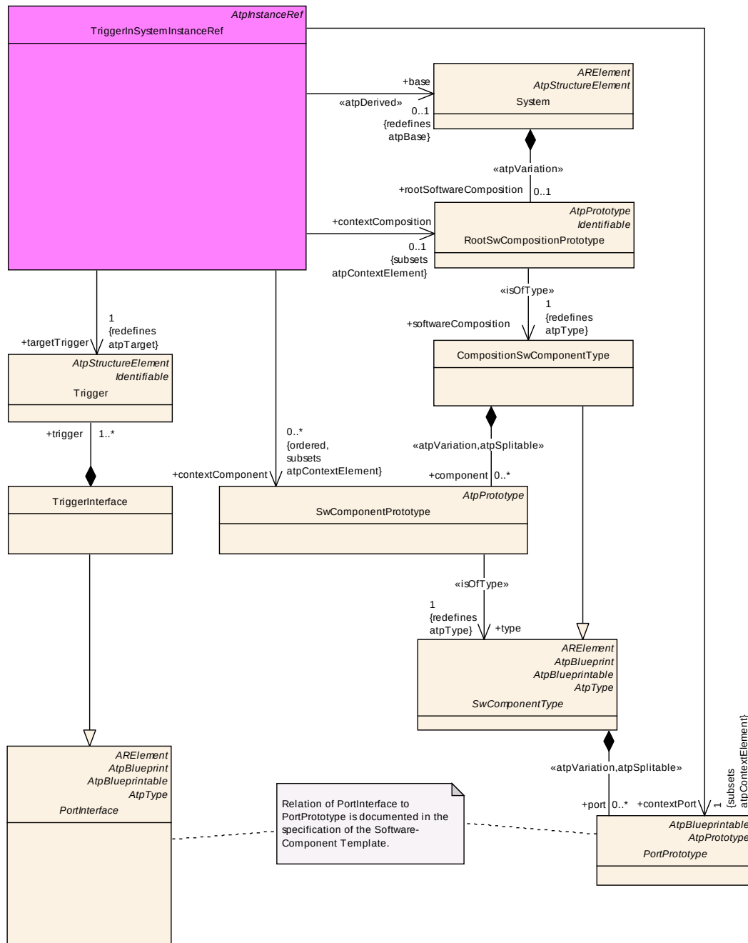
Figure C.9: TriggerInSystemInstanceRef
