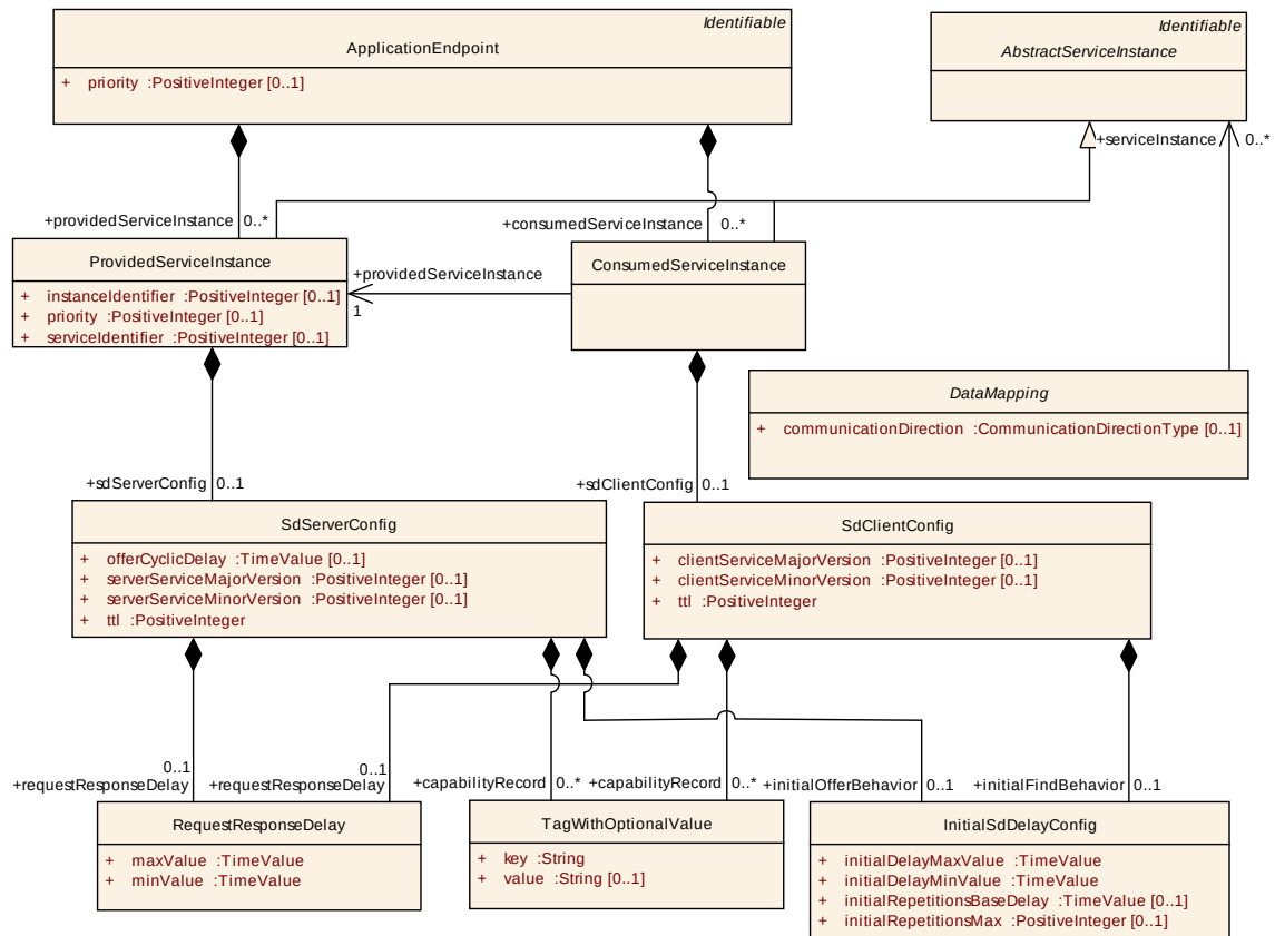
Figure 6.30: Service Instances
