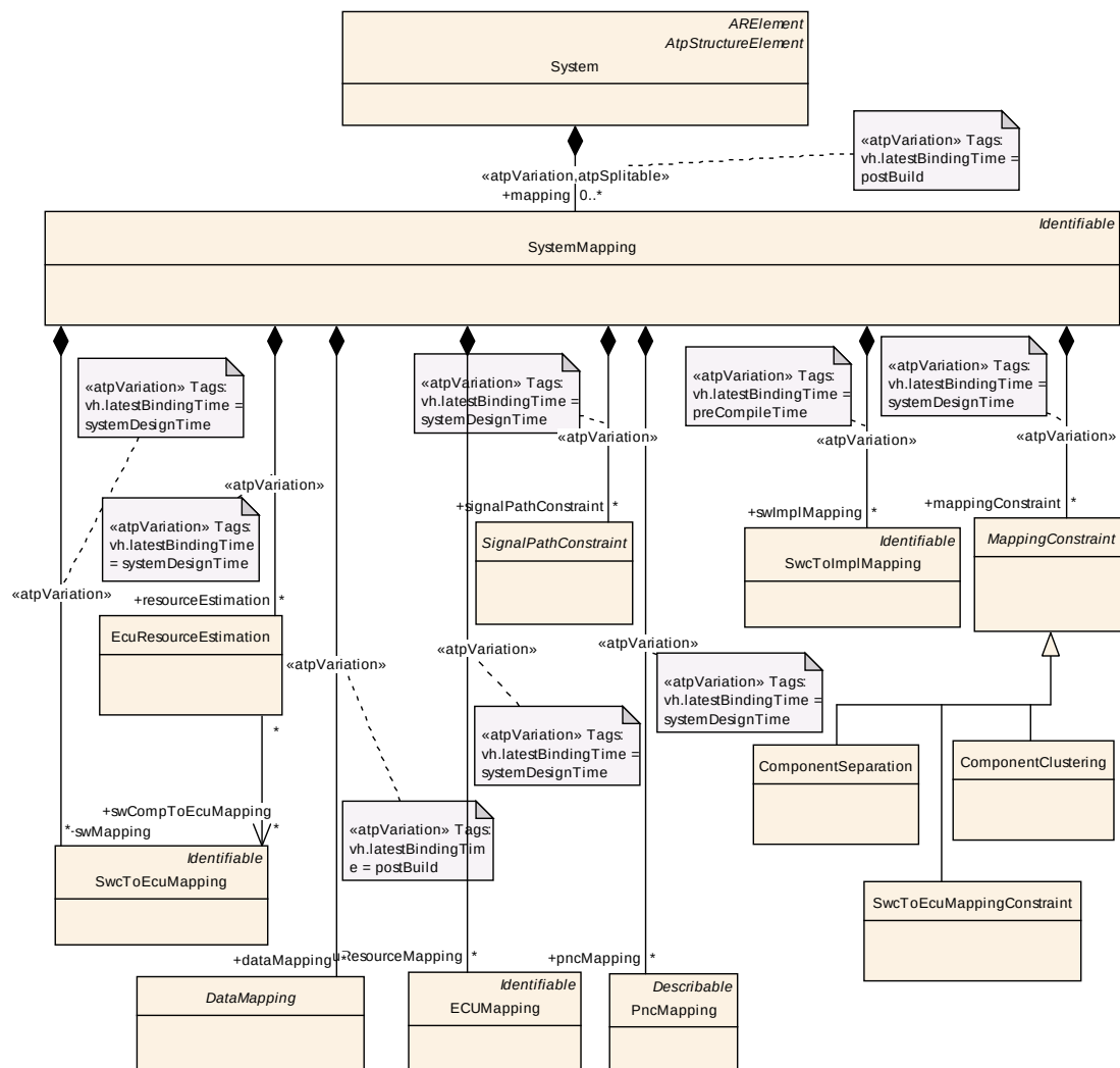
Figure 5.1: Mapping Overview (Mapping)
