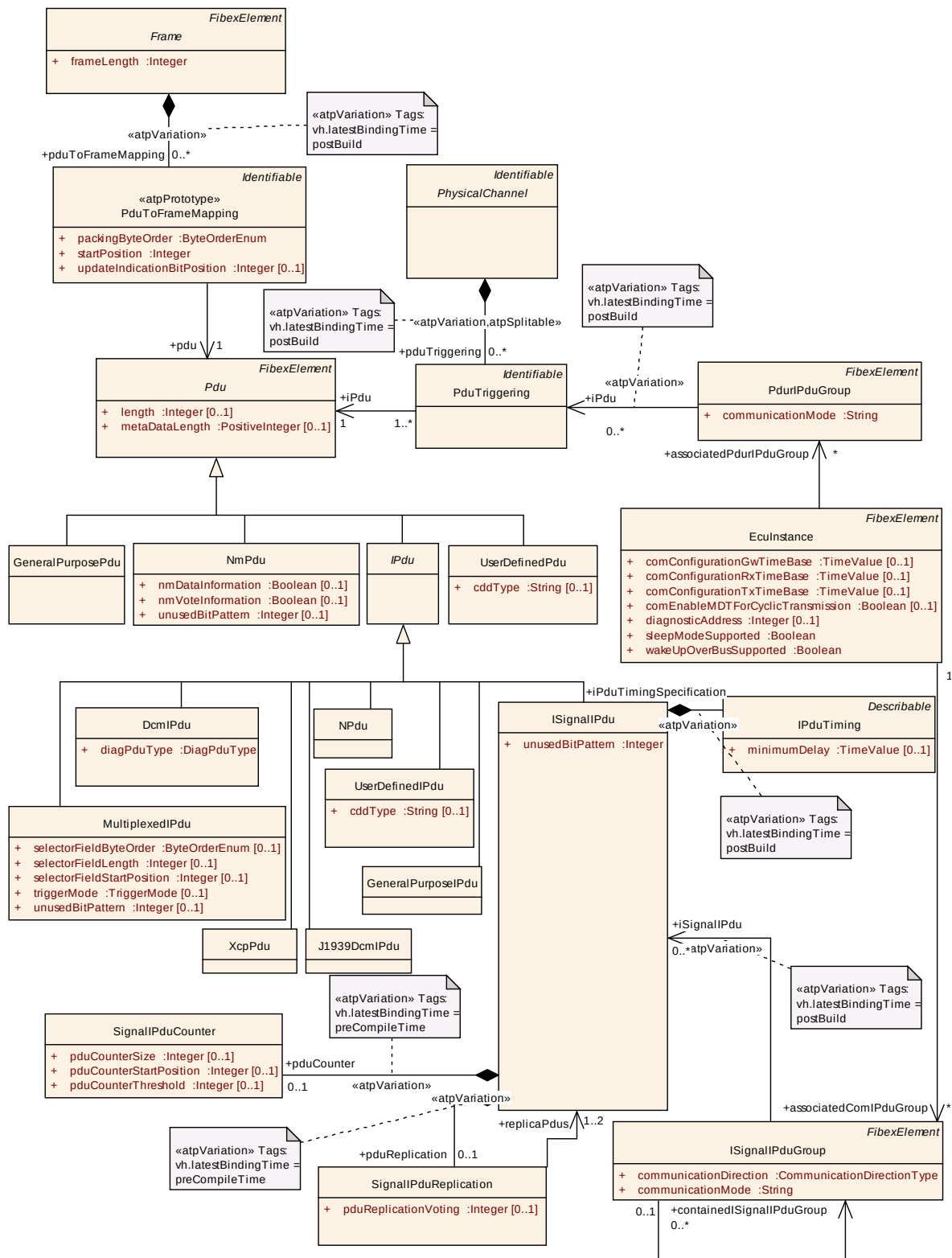
Figure 6.7: Pdus and the mapping into Frames (FibexCore: PDUOverview)
