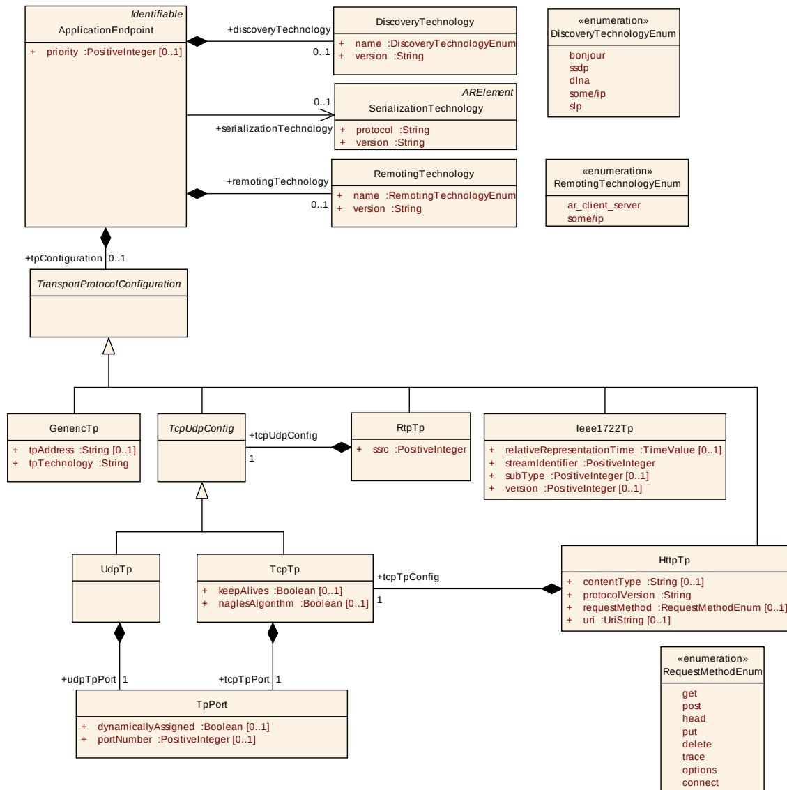
Figure 6.29: Application Endpoint
