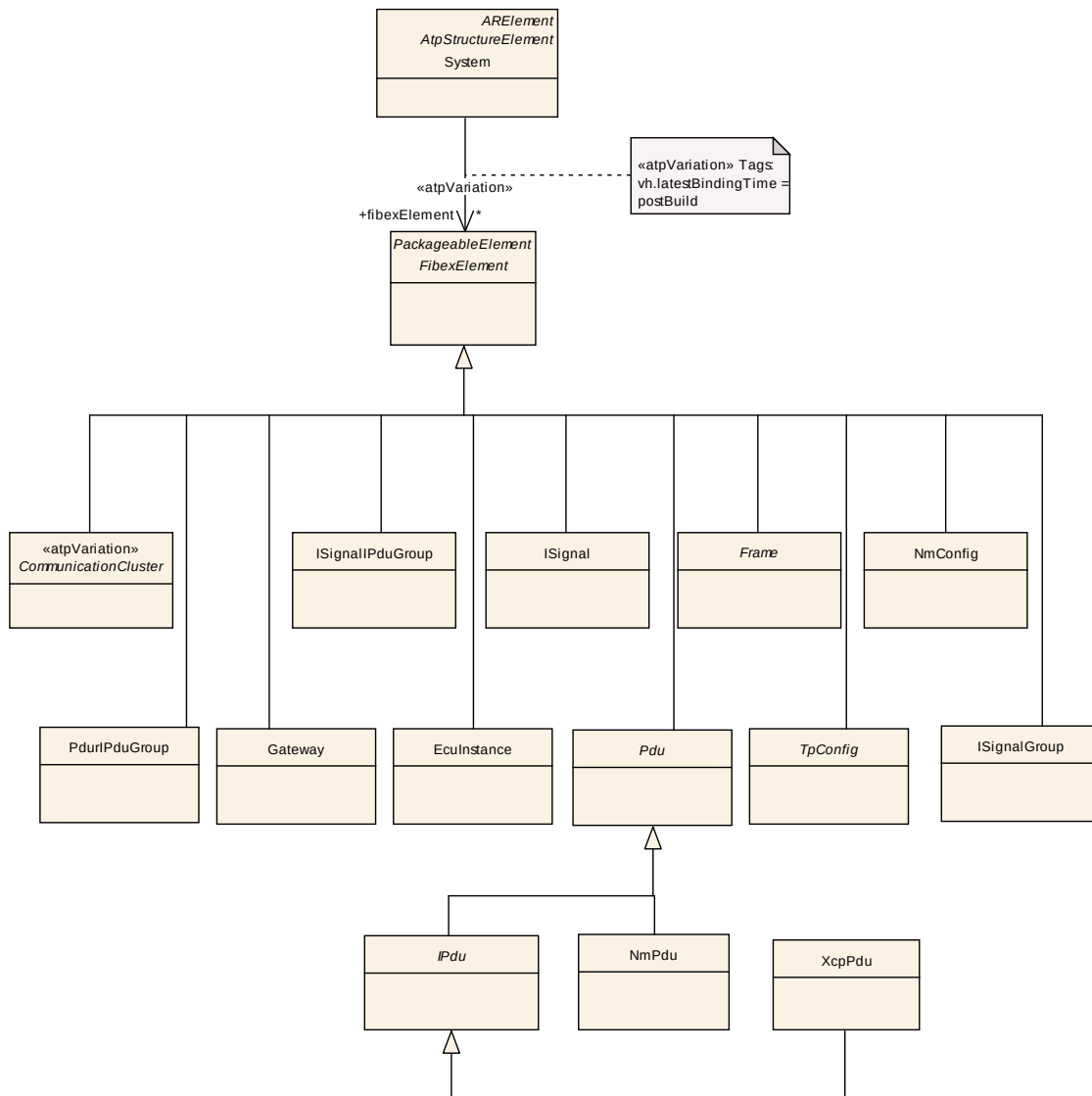
Figure 1.6: Fibex Elements
