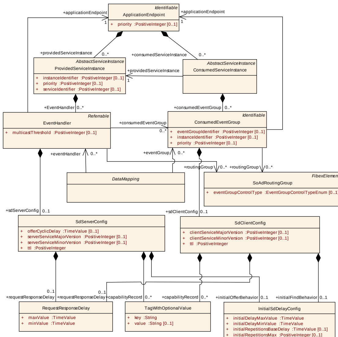
Figure 6.31: Event Handler
