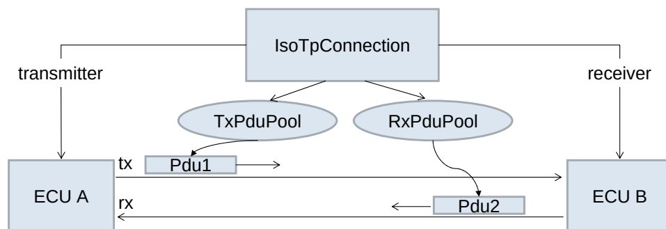
Figure 6.34: IsoTp Example
