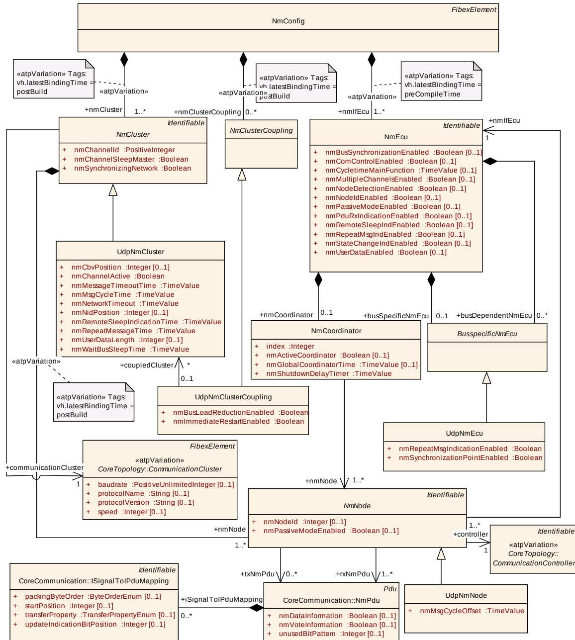
Figure 6.44: UDP Network Management Configuration (TransportProtocols: NmUdpConfiguration)
