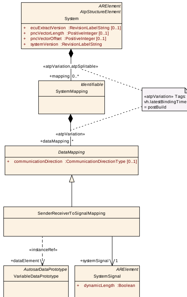
Figure 5.8: Mapping of data elements with primitive datatypes (SenderRecPrimitiveTypeMapping)
