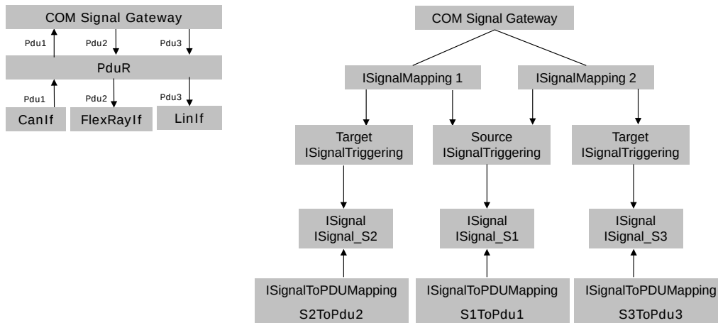
Figure 6.47: Com Gateway fan-out
