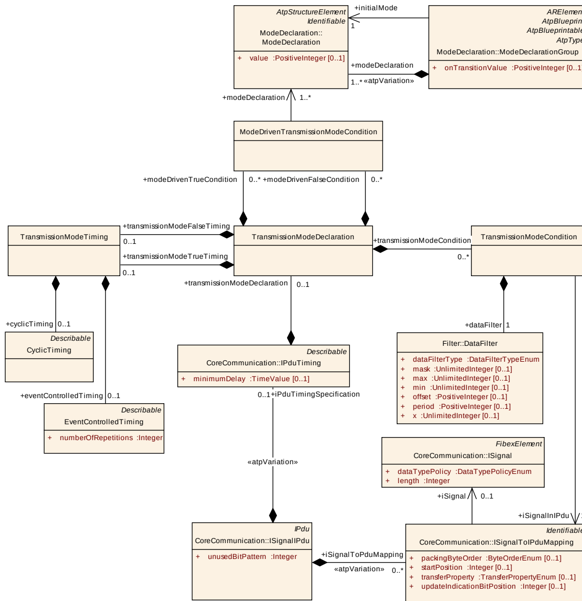
Figure 6.9: IPdu Timing
