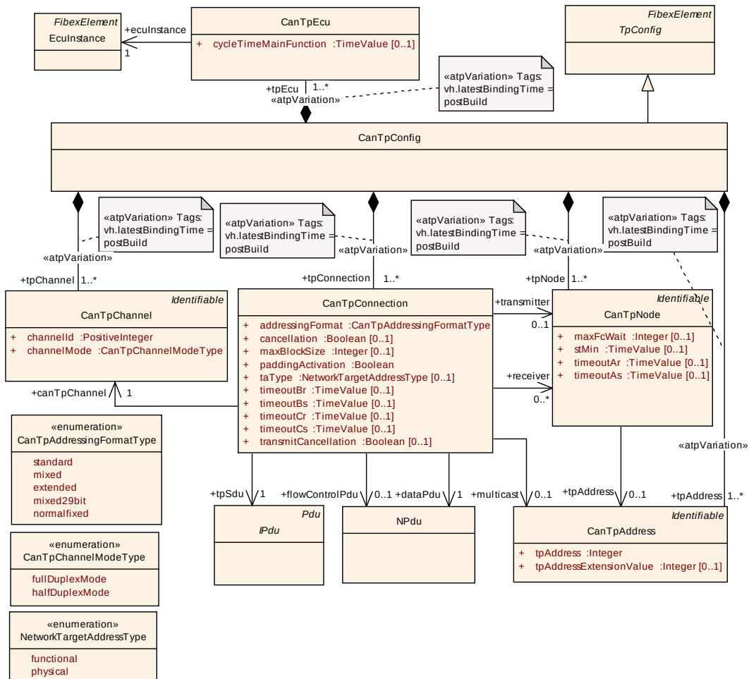
Figure 6.36: CAN Transport Layer Configuration (TransportProtocols: CanTransportProtocol)
